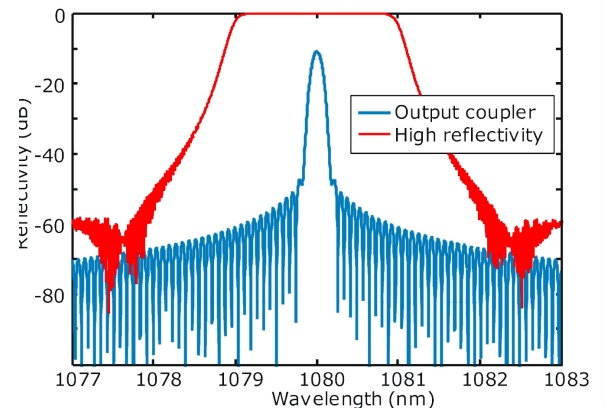
Typical spectrum
